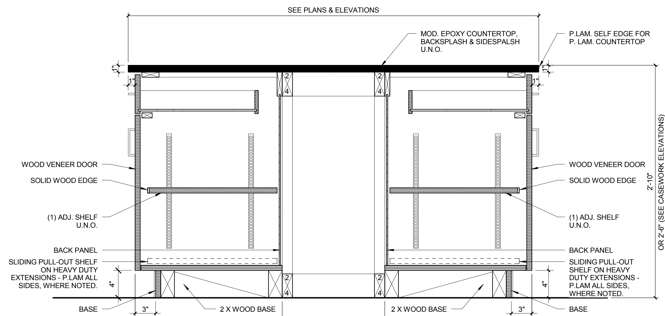
13 BASE CABINET DETAIL - ISLAND_DRAWER+DOOR 1 1/2" = 1'-0"
