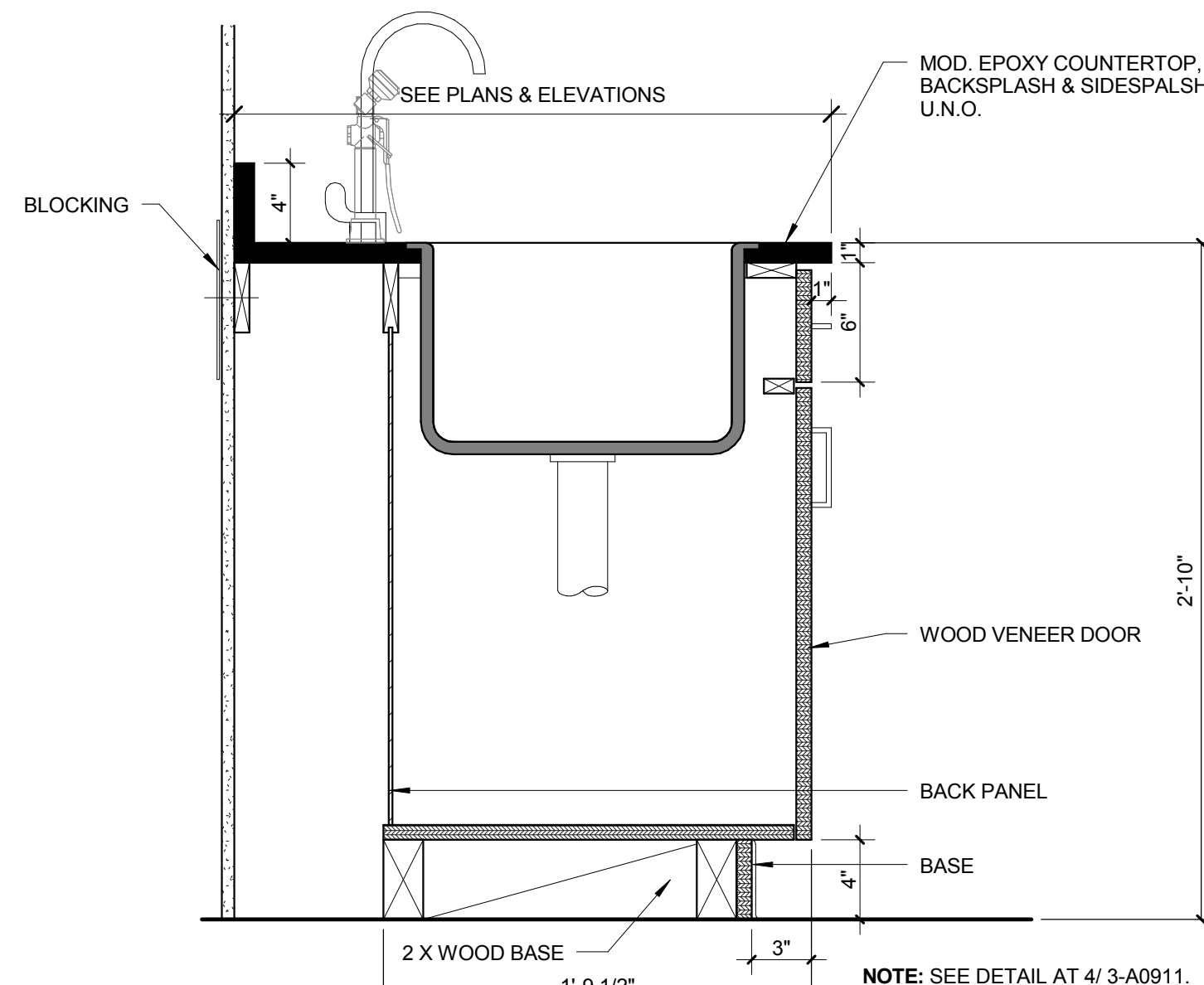
7 BASE SINK CABINET DETAIL 1 1/2" = 1'-0"
