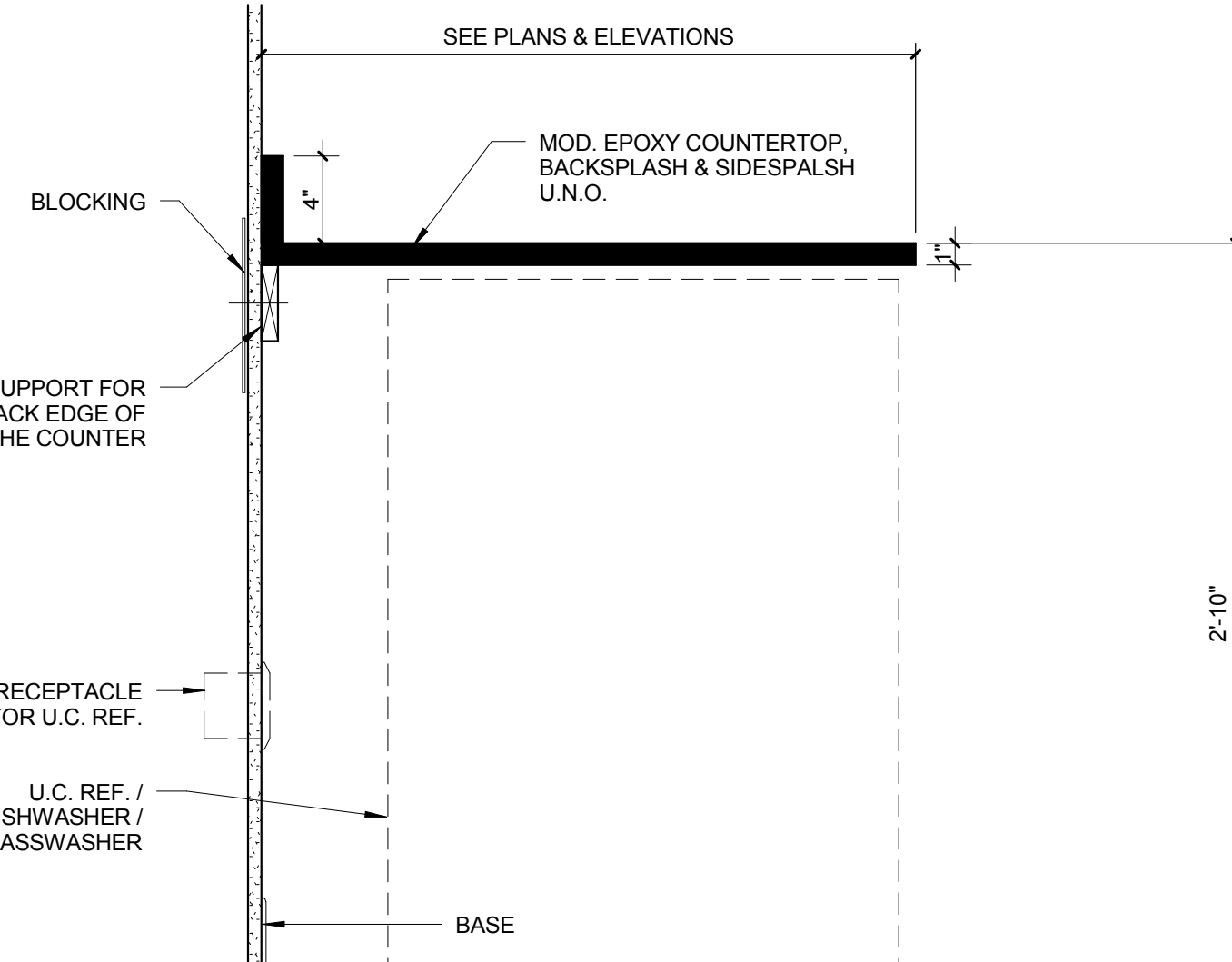
10 CASEWORK DETAIL - U.C. REF. 1 1/2" = 1'-0"
