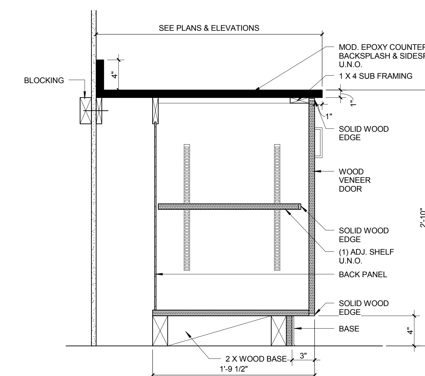
1 BASE CABINET DETAIL 1 1/2" = 1'-0"
