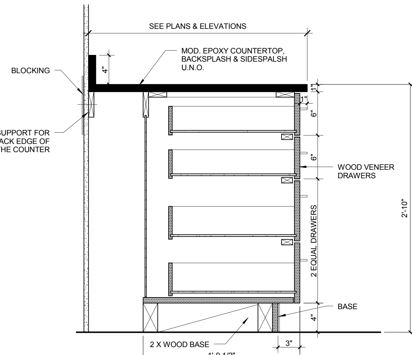
6 BASE CABINET DETAIL - DRAWERS(4) 1 1/2" = 1'-0"
