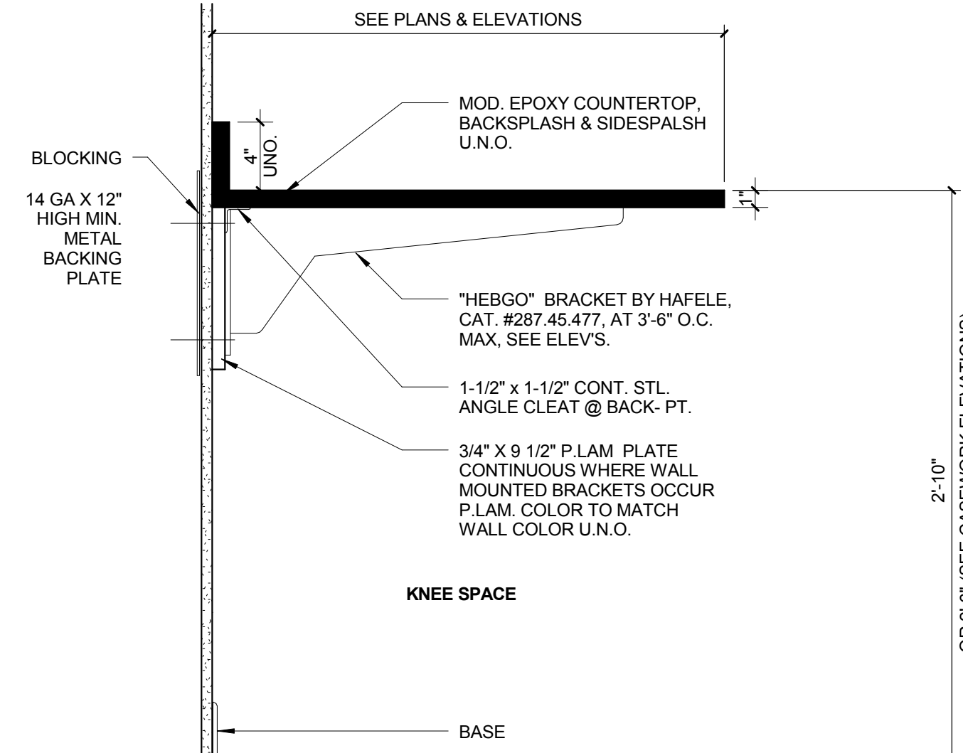
9 CASEWORK DETAIL - METAL BRACKET 1 1/2" = 1'-0"
