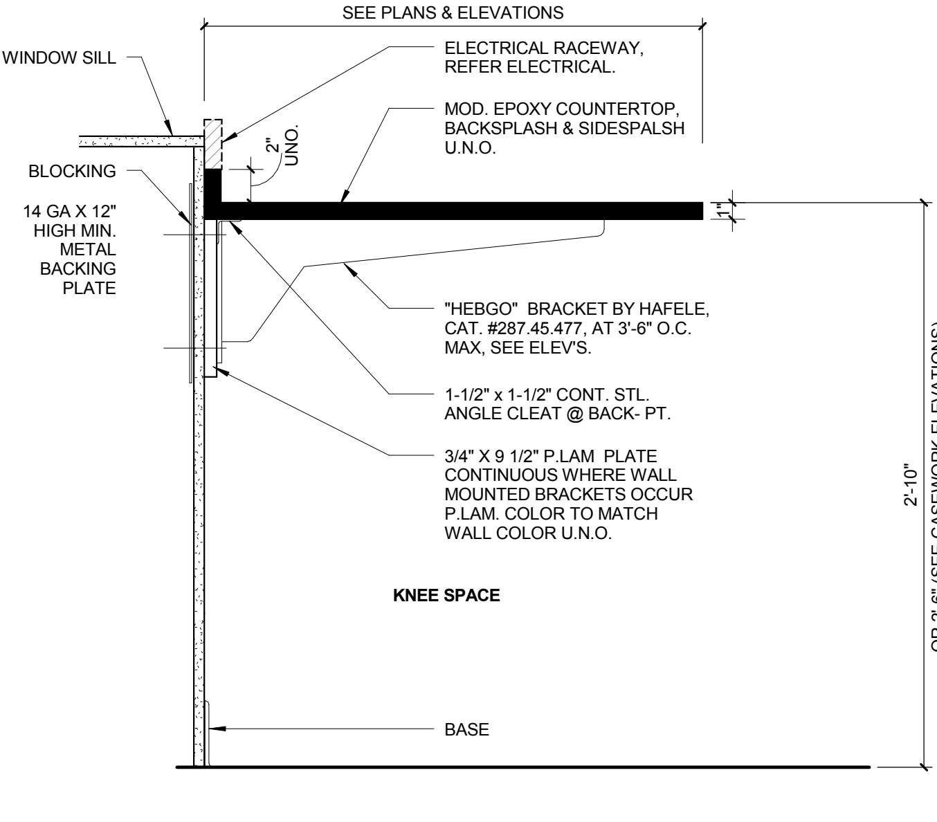
5 CASEWORK DETAIL - METAL BRACKET @ EAST WALL 1 1/2" = 1'-0"
