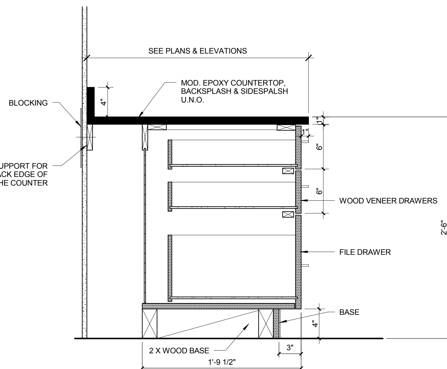
3 BASE CABINET DETAIL - DRAWERS(2) +FILE DRAWER 1 1/2" = 1'-0"
