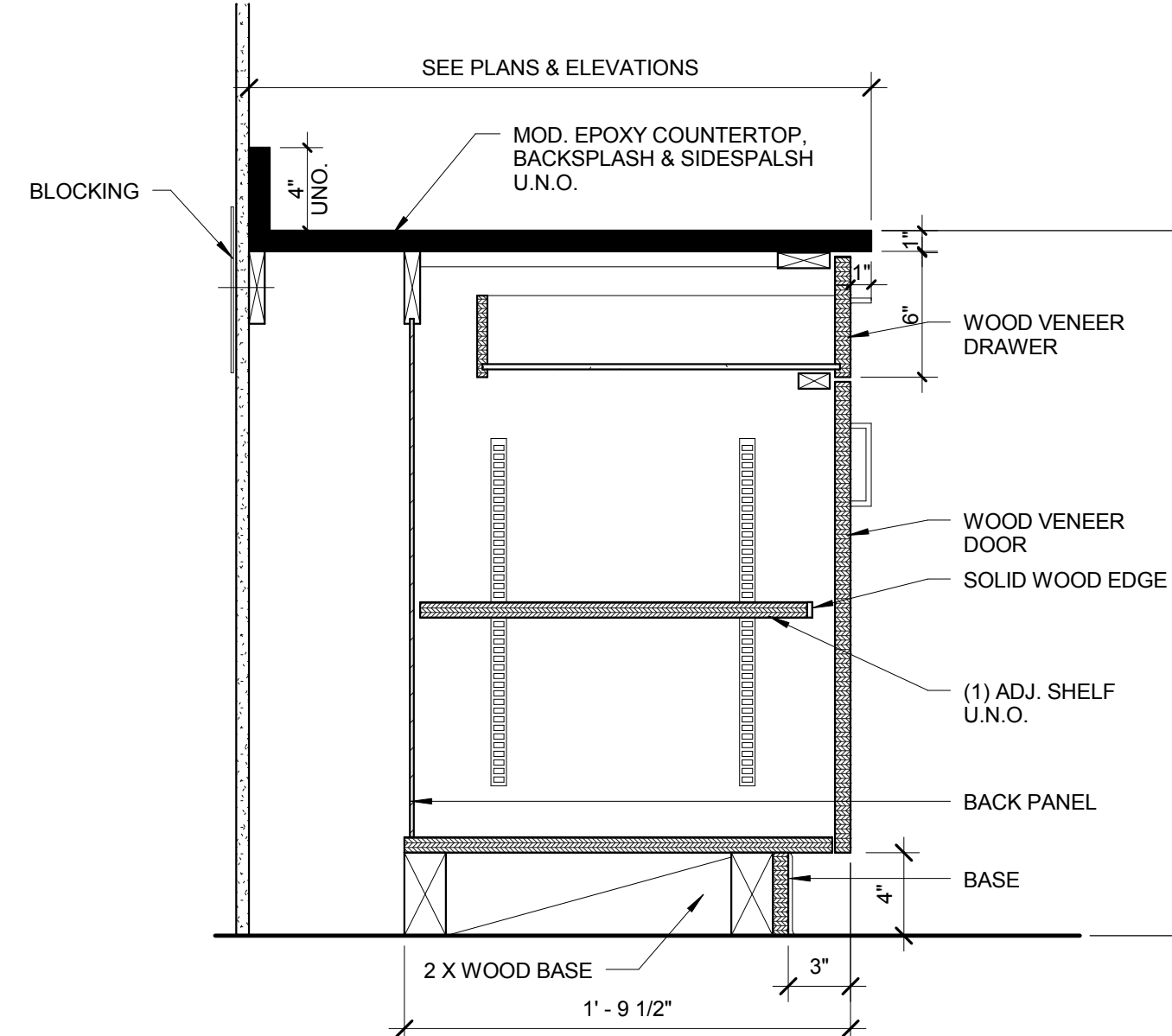
2 BASE CABINET DETAIL - DRAWER+DOOR 1 1/2" = 1'-0"
